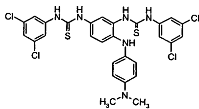
Compound # 35
